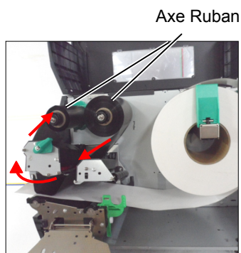
Ruban encre externe
